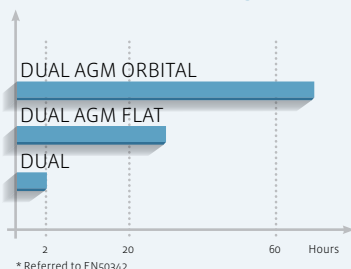
DUAL & DUAL AGM Vibration resistance at 6g/35Hz*
