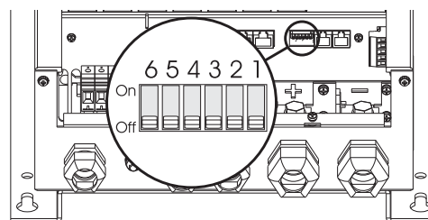
Figure 9: Cavaliers boîtiers C2 et C3 enclosure
